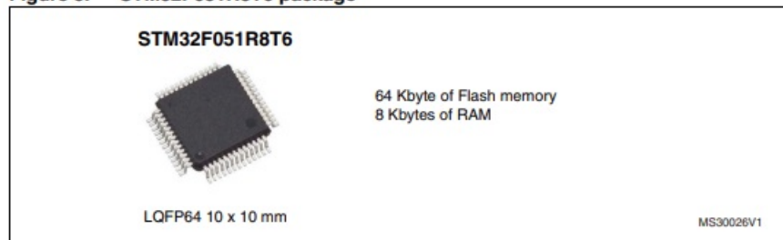
Figure 5. STM32F051R8T6 package
