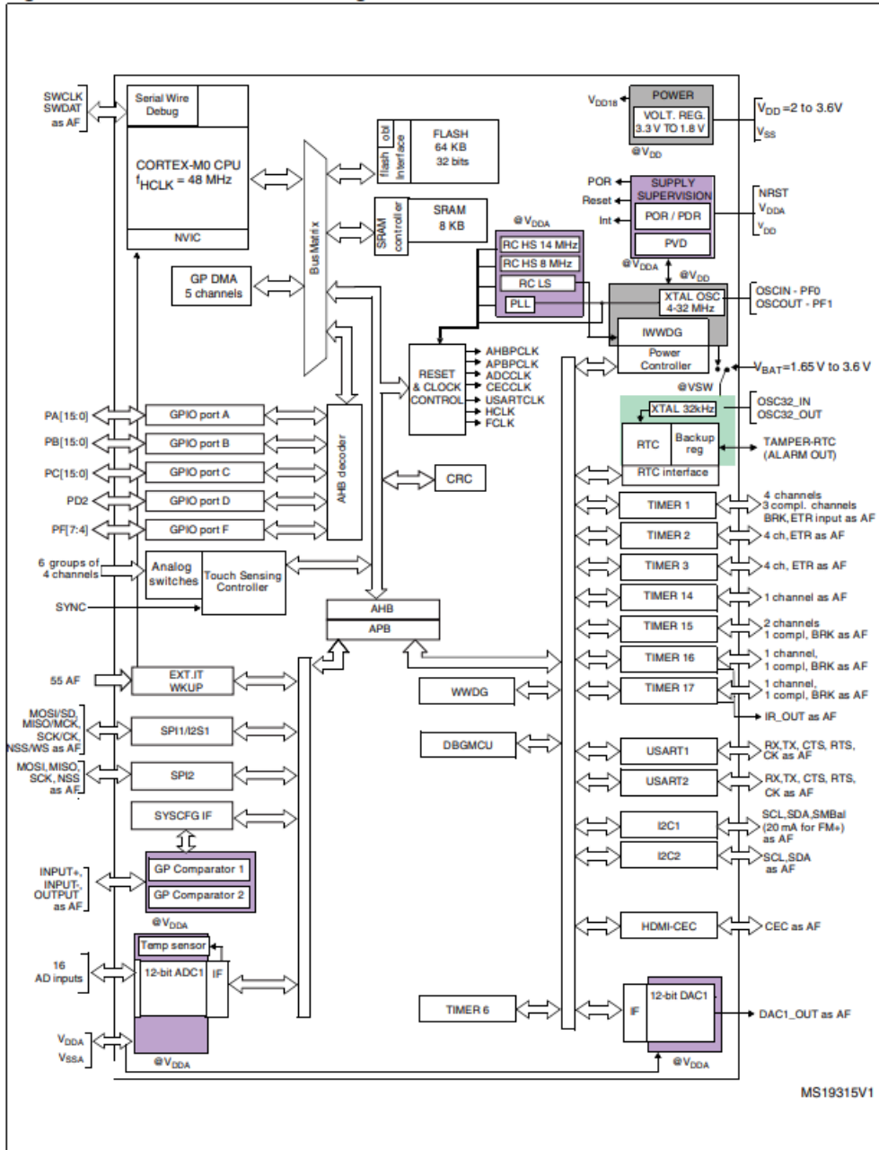
Figure 6. STM32F051R8T6 block diagram
