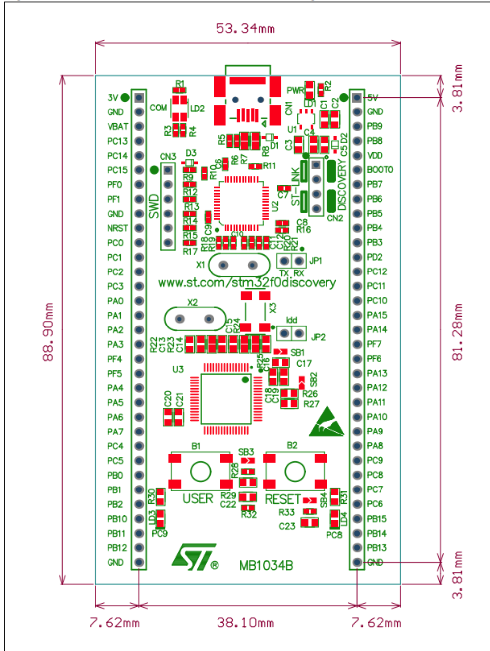
Figure 13. STM32F0DISCOVERY mechanical drawing
